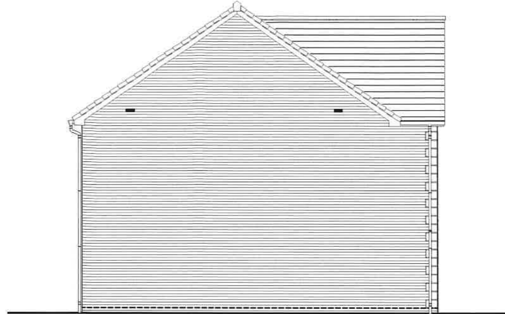
Left Elevation
